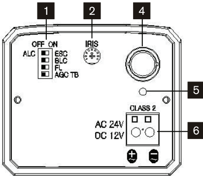
VTC-C750
