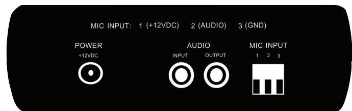
Rear Input Connections
